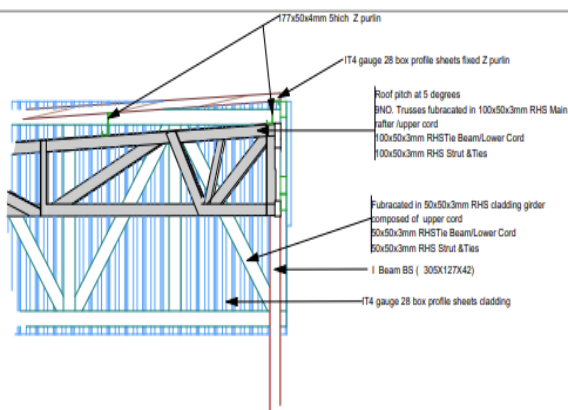
Detail (R)
