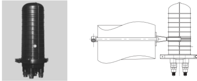
Figure 4 Plastic Splice/Joint Box
