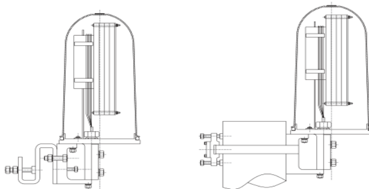
Figure 5 Metal Splice/Joint Box
