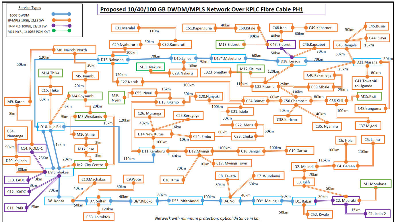
Diagram 1: Proposed DWDM/ MPLS solution for KPLC broadband network
