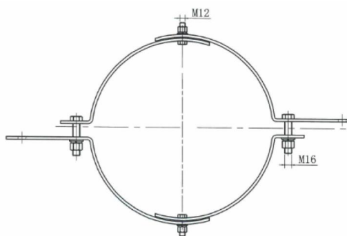
Figure 1 Adjustable Universal Pole Clamp
