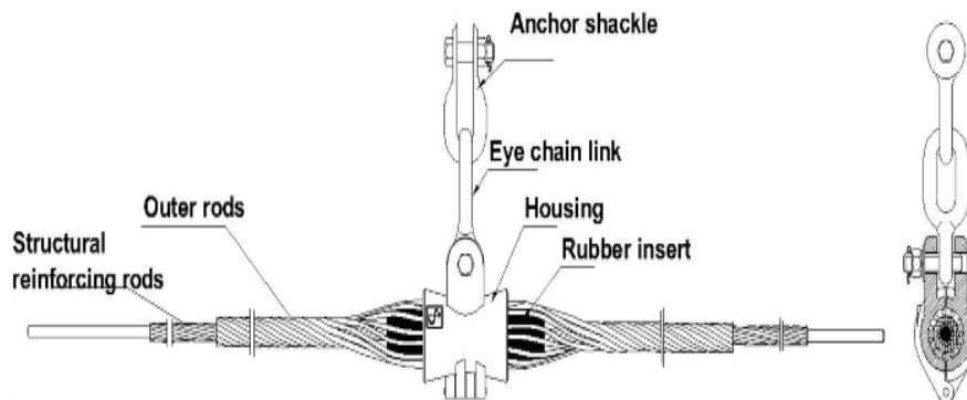
Figure 3 ADSS Suspension Fittings
