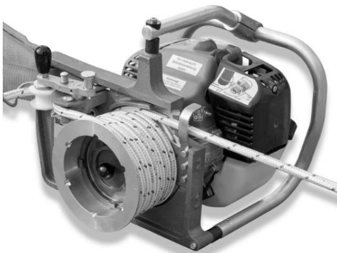
Figure 12: Capstan Winch
