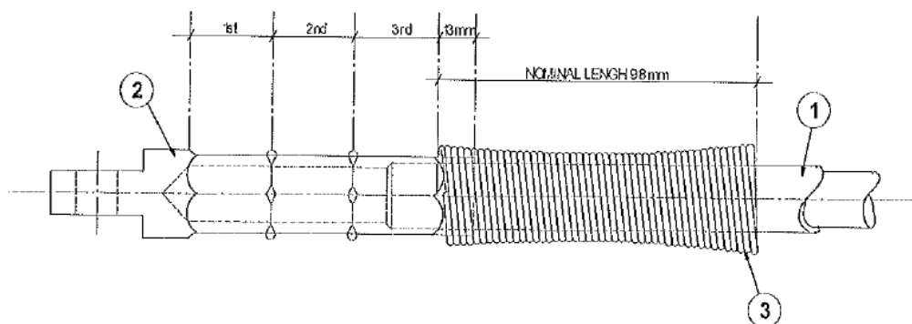
Figure 4: Cable Terminations
